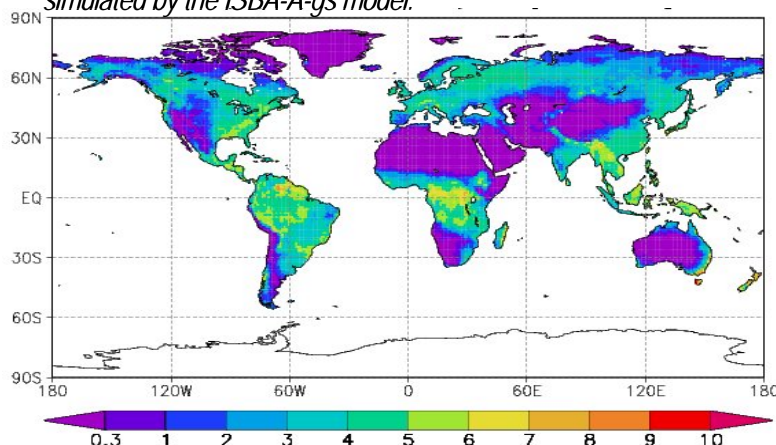
Yearly Maximum of Leaf Area Index (mean 1986-1995) simulated by the ISBA-A-gs model.
